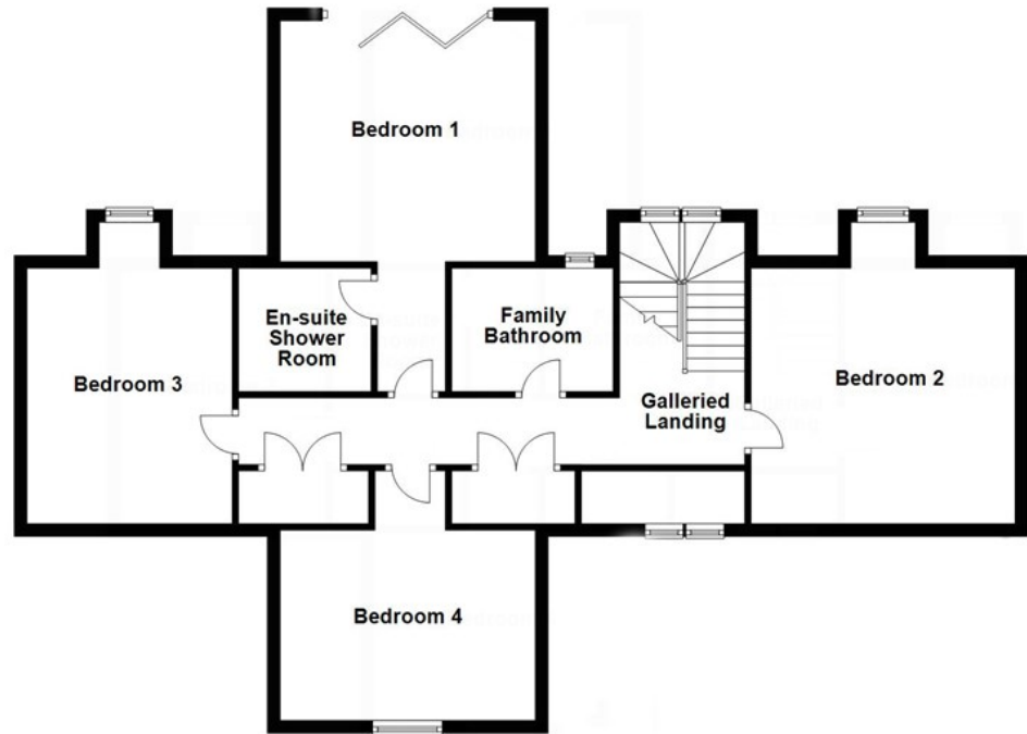
First Floor
